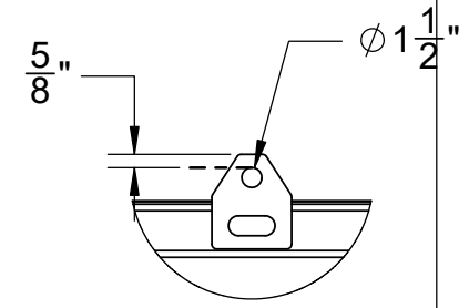
DETAIL A SCALE 1 : 16 5/8" A36 Plate
